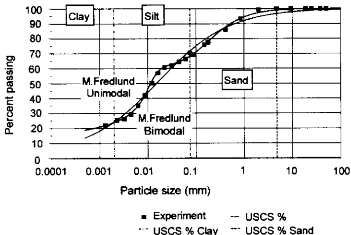
Fig. 10 Example of a bimodal fit of a gap-graded Saprolitic Soil tested at the University of Saskatchewan ( R^2 = 0.999 )
