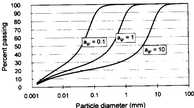
Fig. 4 Effect of varying the a_{gr} parameter while n_{gr} = 4.0 , m_{gr} = 0.5 , d_{rgr} = 100 and d_m = 0.001 .
