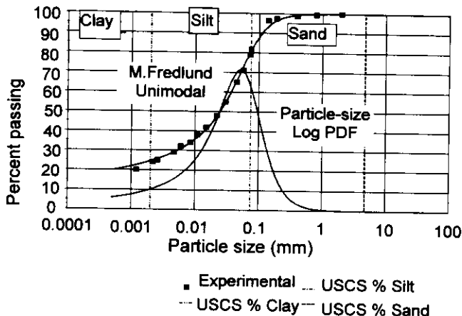
Fig. 2 Logarithmic probability density function for uniform silt from the Pilot Butte area of Saskatchewan (optimum compression) best fit with the unimodal equation.
