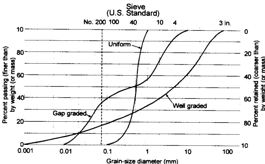
Fig. 1 Three primary types of grain-size distribution curves (Holtz and Kovacs, 1981)
