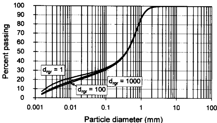
Fig. 7 Effect of varying the d_{rgr} parameter while a_{gr} = 1.0 , n_{gr} = 4.0 , m_{gr} = 0.5 , and d_m = 0.001
