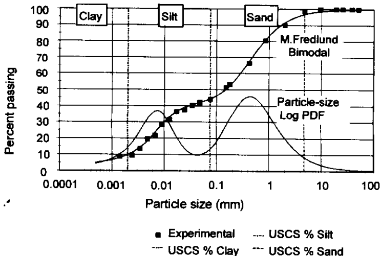
Fig. 8 Logarithmic probability density function fitted with a bimodal equation, for a gap-graded Saprolitic Soil tested at the University of Saskatchewan
